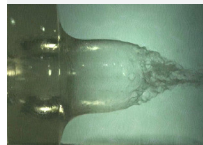
Full pass-through with devastating trauma
